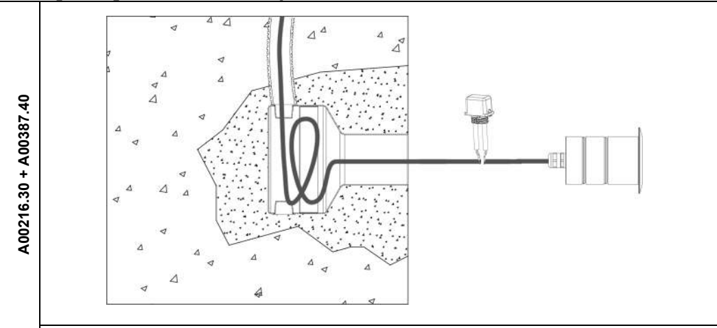
COLLEGAMENTO STAGNO INTERNO - INTERNAL SEALED CONNECTIONS
