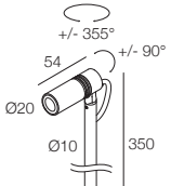
A Stake H350
