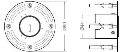
Frame for trimless installation
