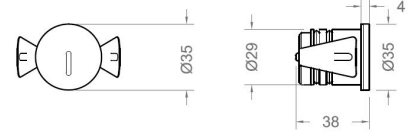
Spring mounting support
