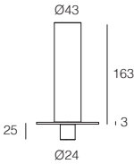
Stainless Steel IP68 recessed box A01086.60
